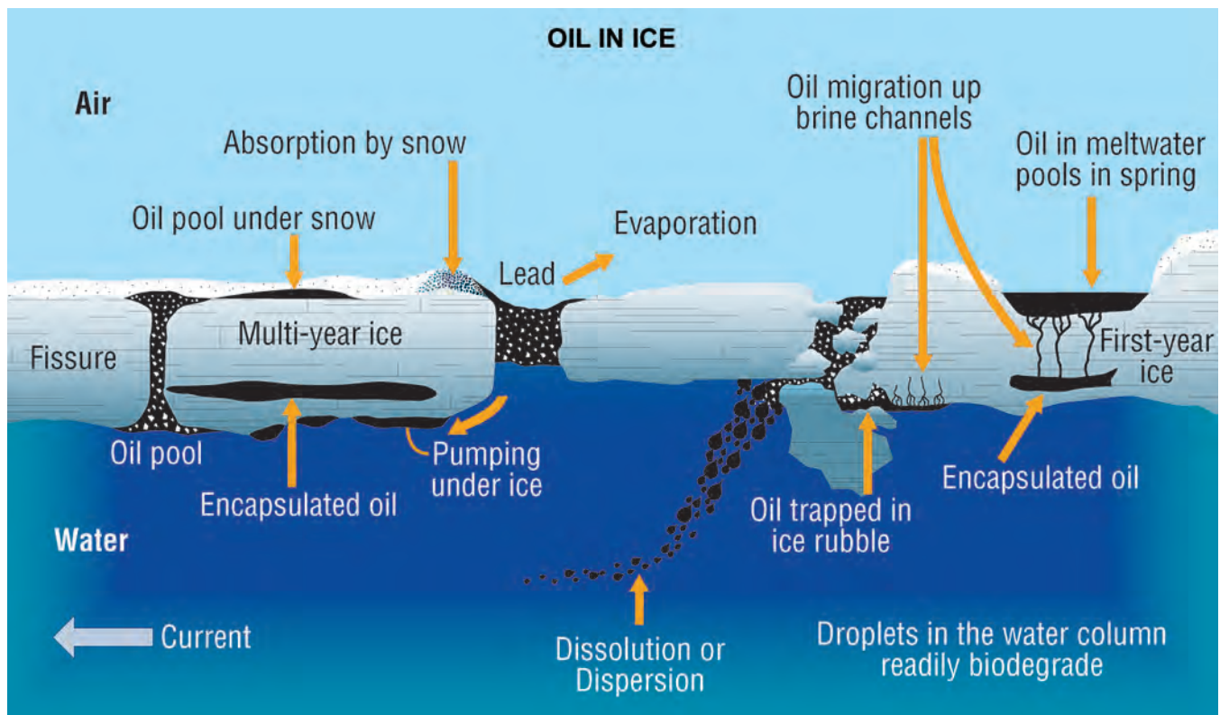
Figure 8-9. Depiction of Oil Interacting with Ice
