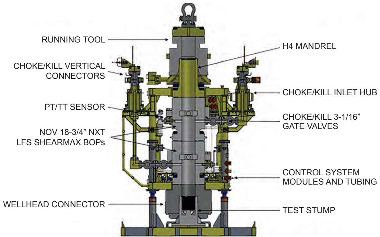
Figure 8-6. Internal View of a Subsea Shut-In Device
