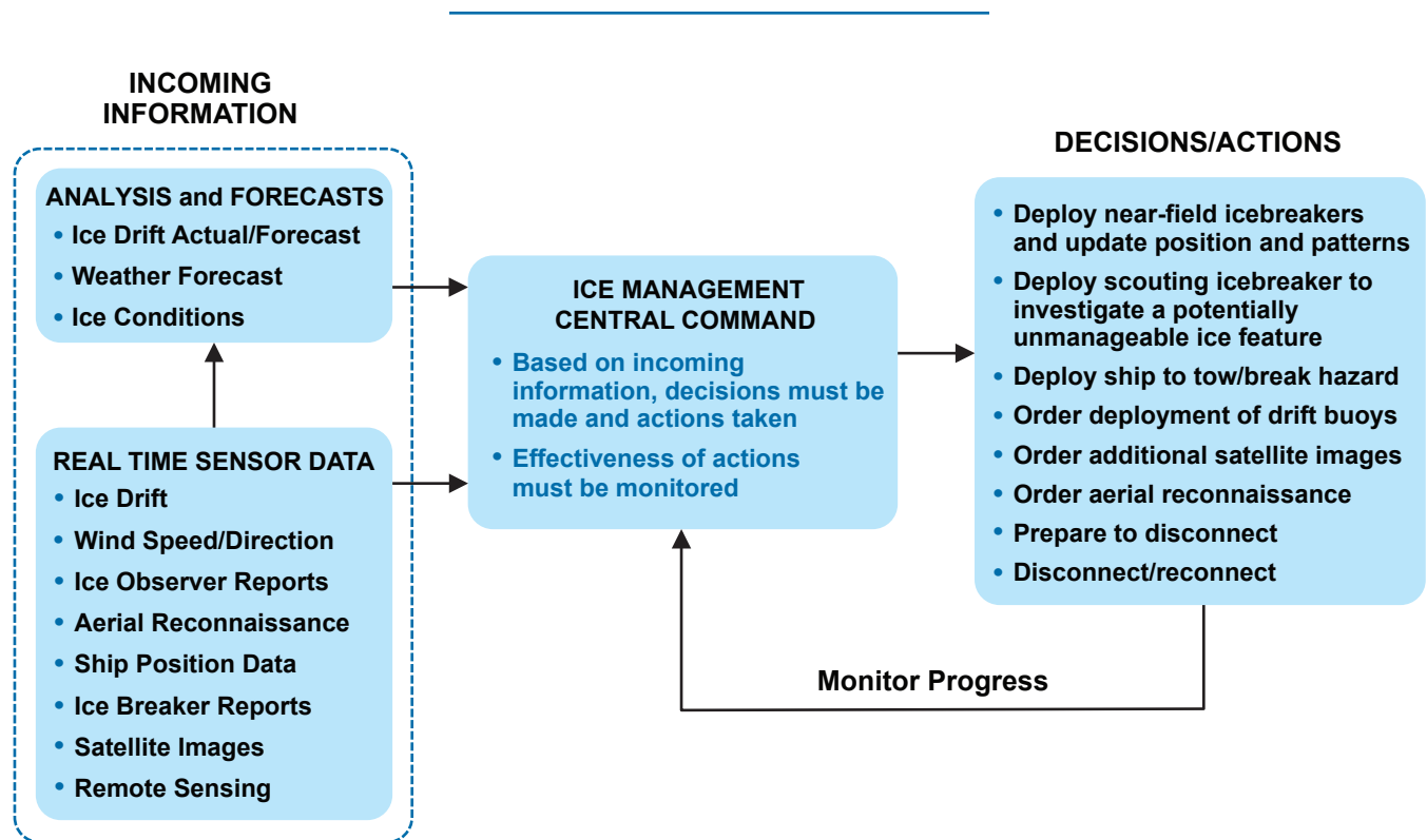
Figure 6-14. Schematic of an Integrated Ice Management Program
