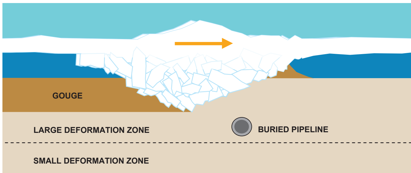
Figure 6-23. Ice Gouging Process
