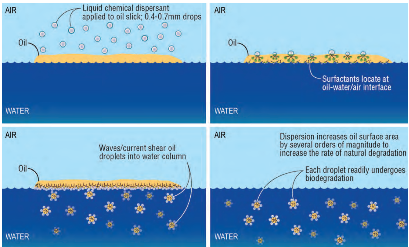
Figure 8-11. Schematic Drawing Illustrates the Dispersion Process
