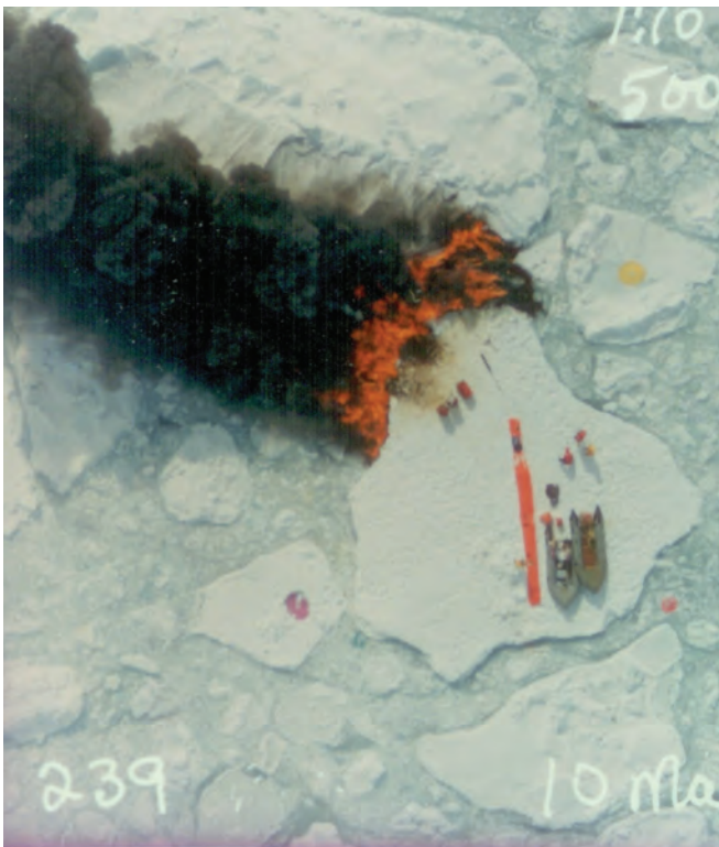
Figure 8-14. Aerial and Surface Views of Burning Crude Oil Spilled in Slush Between Floes During the 1986 Canadian East Coast “Oil in Pack Ice” Experiment
