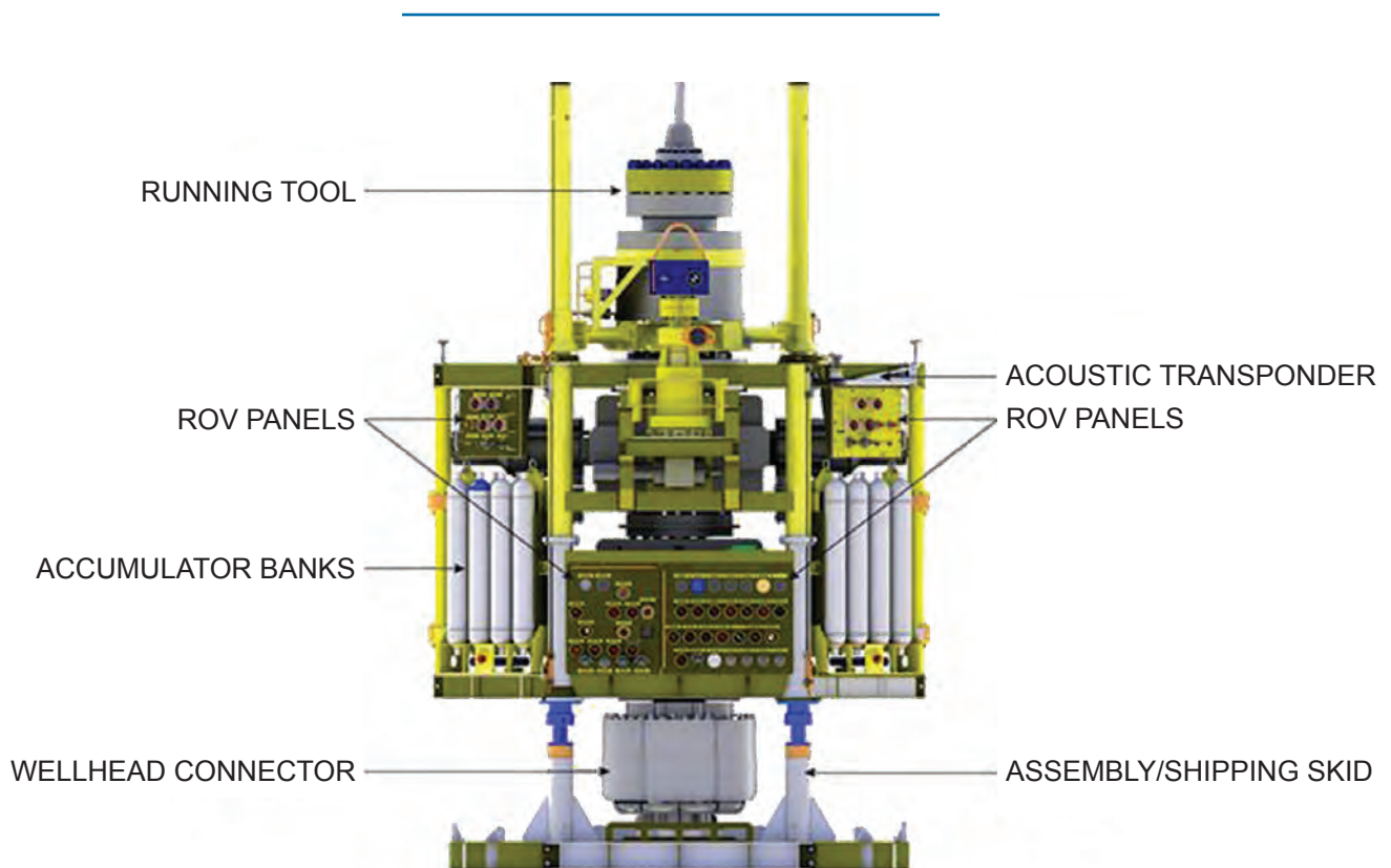
Figure 8-5. External View of a Subsea Shut-In Device
