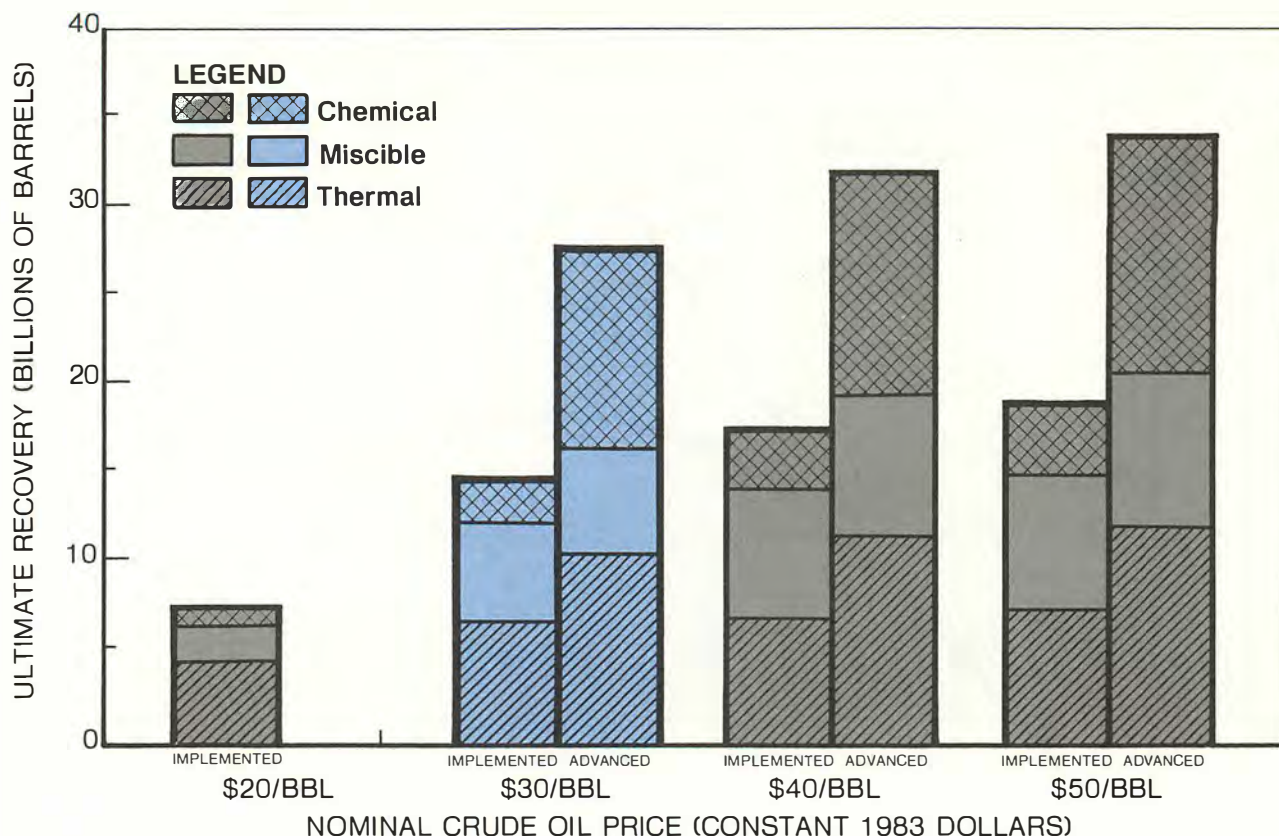
Figure 40. Ultimate Recovery by Process—Advanced and Implemented Technology Cases (10 Percent Minimum ROR).
