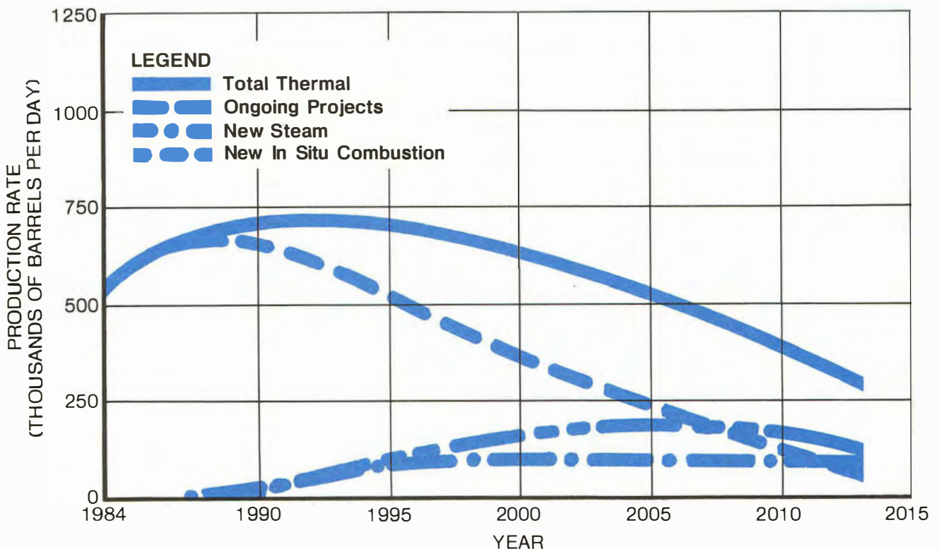
Figure F-7. Production Rate for Thermal Recovery—Implemented Technology, Base Economic Case ($30 per Barrel Nominal Crude Oil Price, 10 Percent Minimum ROR).
