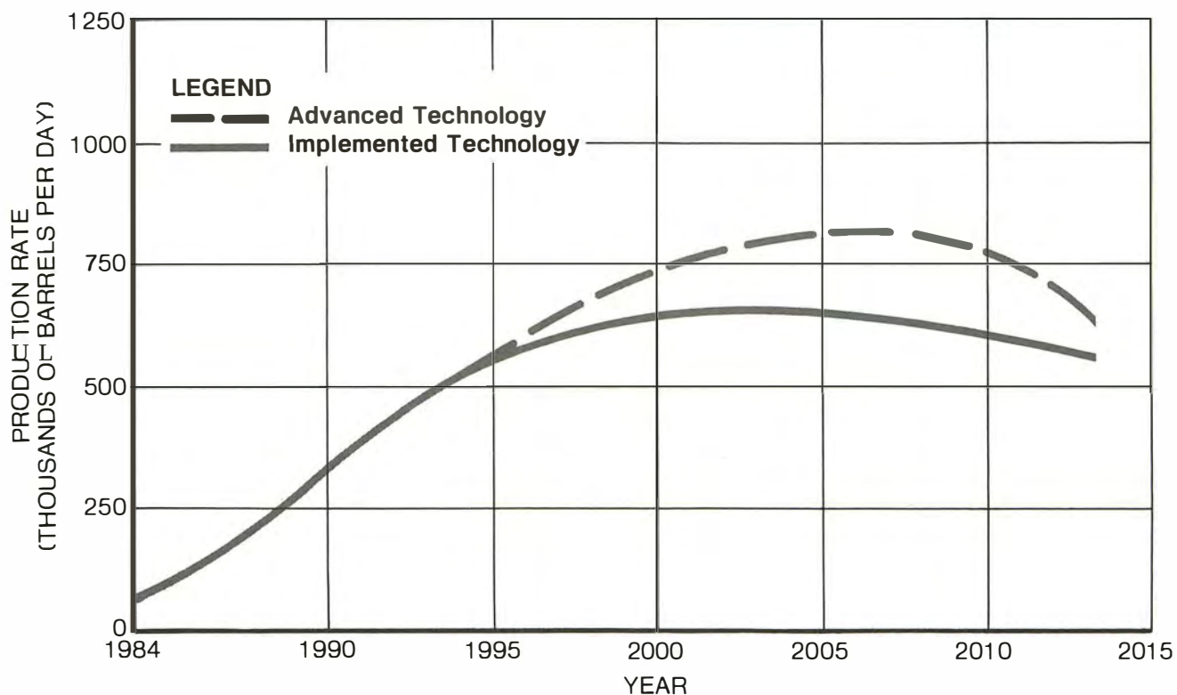
Figure E-15. Comparison of Miscible Flooding Implemented and Advanced Technology Production Rates ($40 per Barrel Nominal Crude Oil Price, 10 Percent Minimum ROR).
