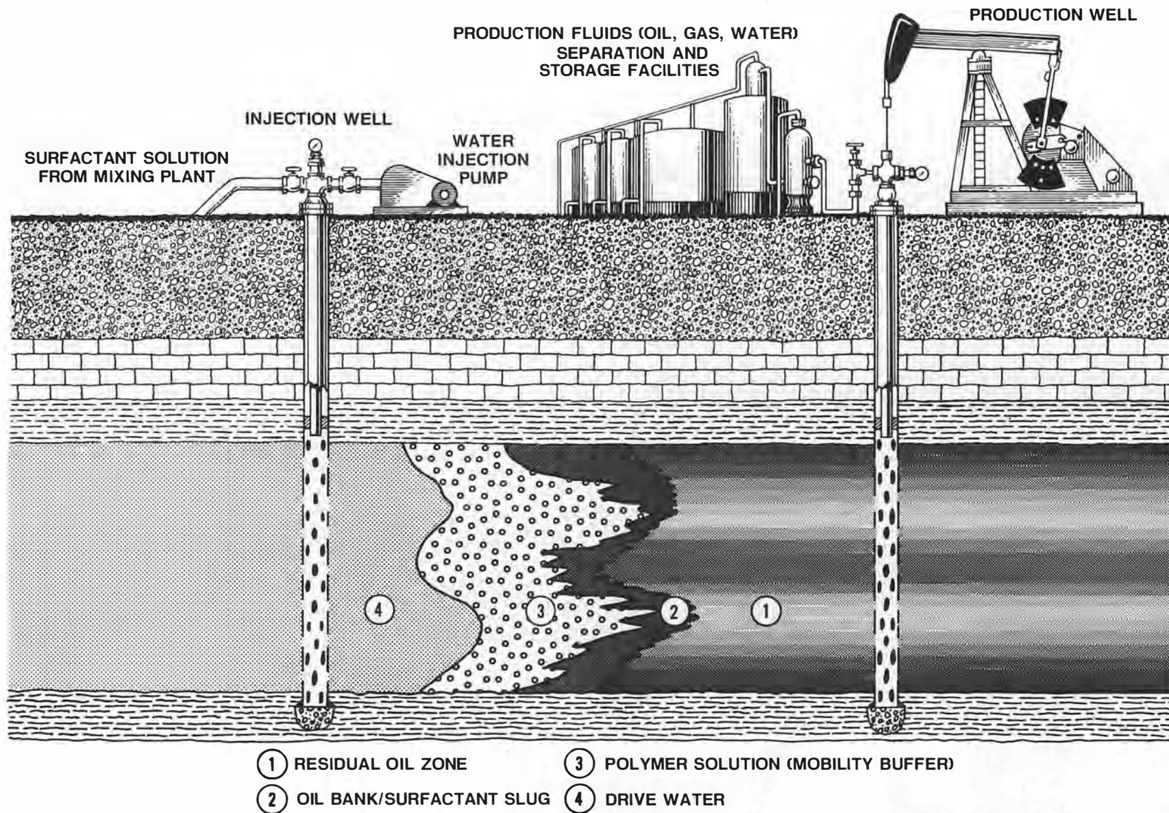
Figure 6. Surfactant Flooding.
