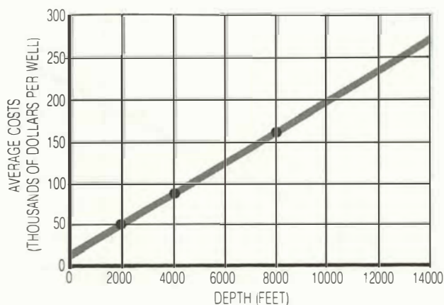
Figure C-19. Cost of Equipping New Producing Wells for the Rocky Mountains, 1982.
